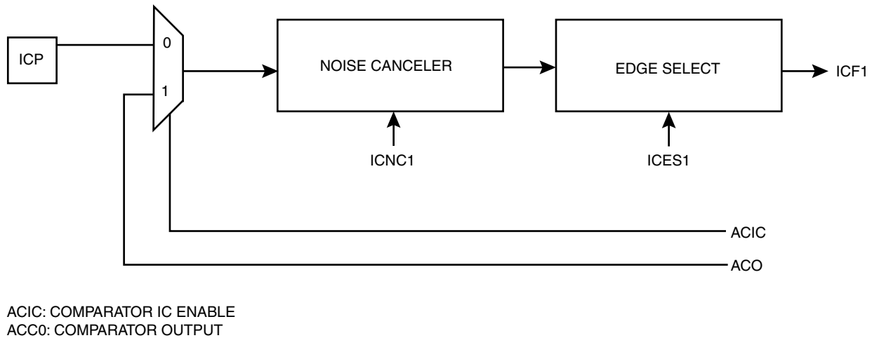
Figure 15. ICP Pin Schematic Diagram
